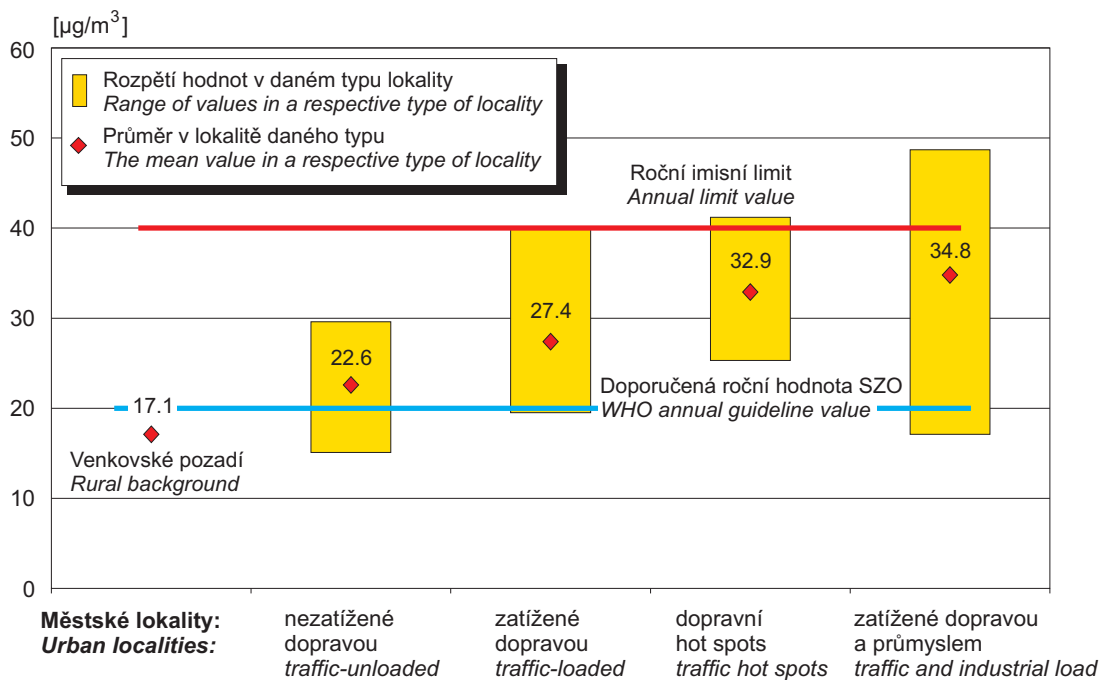
Fig. 2.2b Annual mean levels of particulate matter PM 10 by type of the urban locality, 2008
