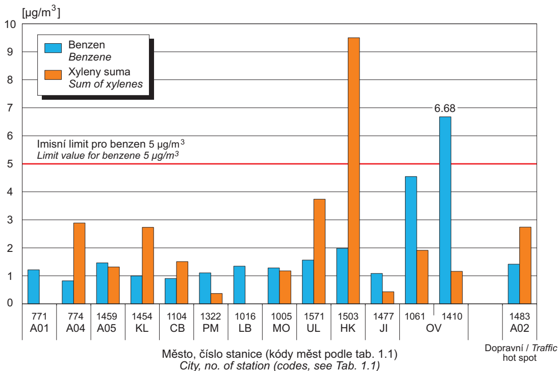
Fig. 2.3a Levels of volatile organic compounds, arithmetic annual mean 2008
